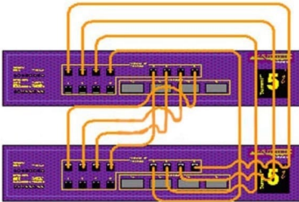
8 port load share group physical connections
